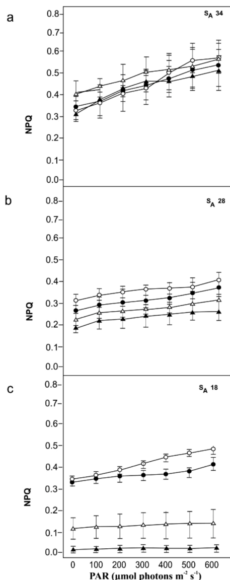
Fig. 3. Mean±SD of NPQ ( n = 3 ) for Palmaria palmata . Measurements plotted for days 1 (circles) and 21 (triangle). Two light points are LL at 50 \mu\text{mol photons m}^{-2} \text{s}^{-1} (black) and HL at 500 \mu\text{mol photons m}^{-2} \text{s}^{-1} (white). Measurements were performed at the three salinities analysed ( S_A 34, 28, and 18).
