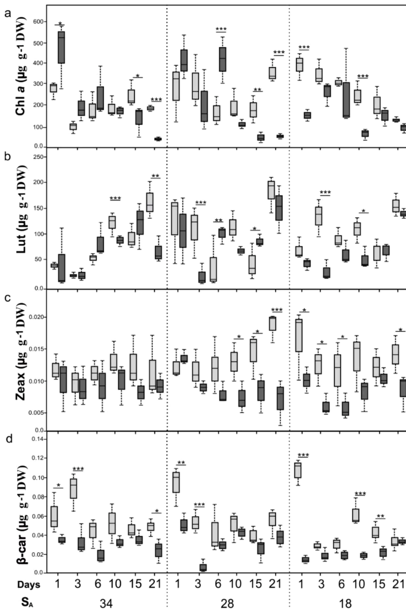
Fig. 4. Mean \pm SD pigment concentration ( n = 3 ) in Palmaria palmata . For pigments, Chlorophyll a (Chl a ), Lutein (Lut), Zeaxanthin (Zeax), and \beta -Carotene ( \beta -Car) in ( \mu\text{g g}^{-1} DW). Samples at three different salinities ( S_A 34, 28, and 18) and two different light points LL at 50 \mu\text{mol photons m}^{-2} \text{s}^{-1} (dark grey) and HL at 500 \mu\text{mol photons m}^{-2} \text{s}^{-1} (light grey). Measurements represented from days 1 to 21. An asterisk indicates statistically significant values between LL and HL: (***) p < 0.0001 , (**) p < 0.001 , (*) p < 0.01 .
